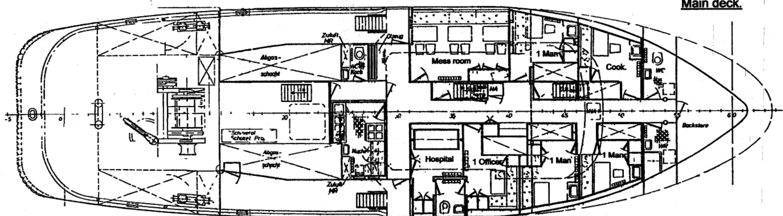
Main deck.
