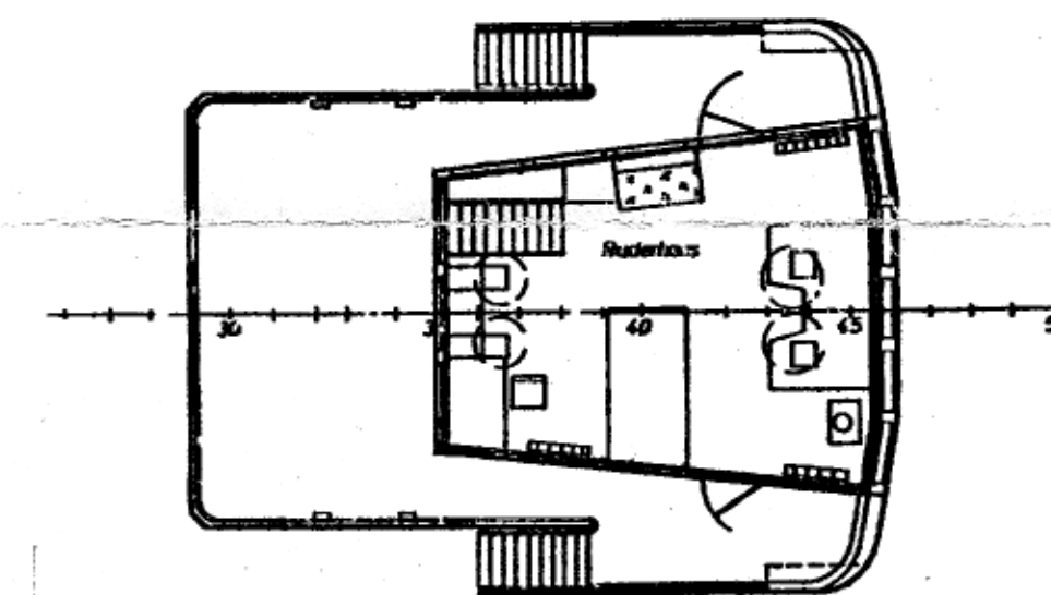
Bridge deck.
